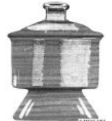
No. 684 - Scheibler Desiccating Jar, Ground Knob Cover with Hole For stoppering. Hand made, heavy weight. Same as 682 except for hole in cover. Inside diameter x inside height sizes: (#1)6"x6", 6"x8 1/2", (#2)8"x8", 8"x11", (#3)10"x9 1/4" & 10"x12 1/2".
